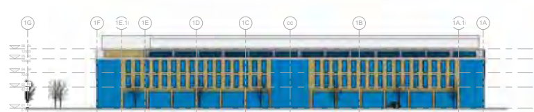
1 01. Front 1:200
