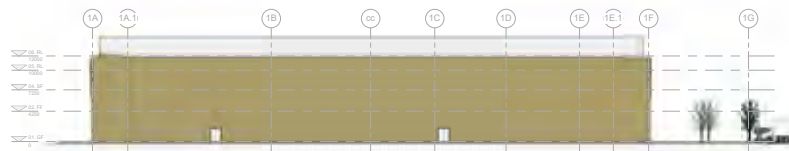
2 02. Rear 1:200
